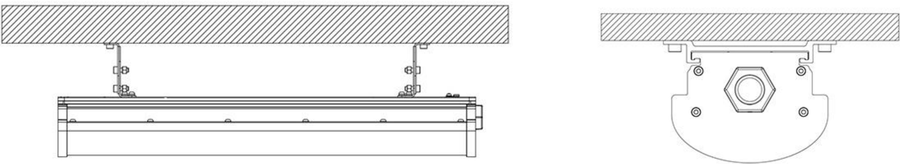
A.Ceiling mounting
