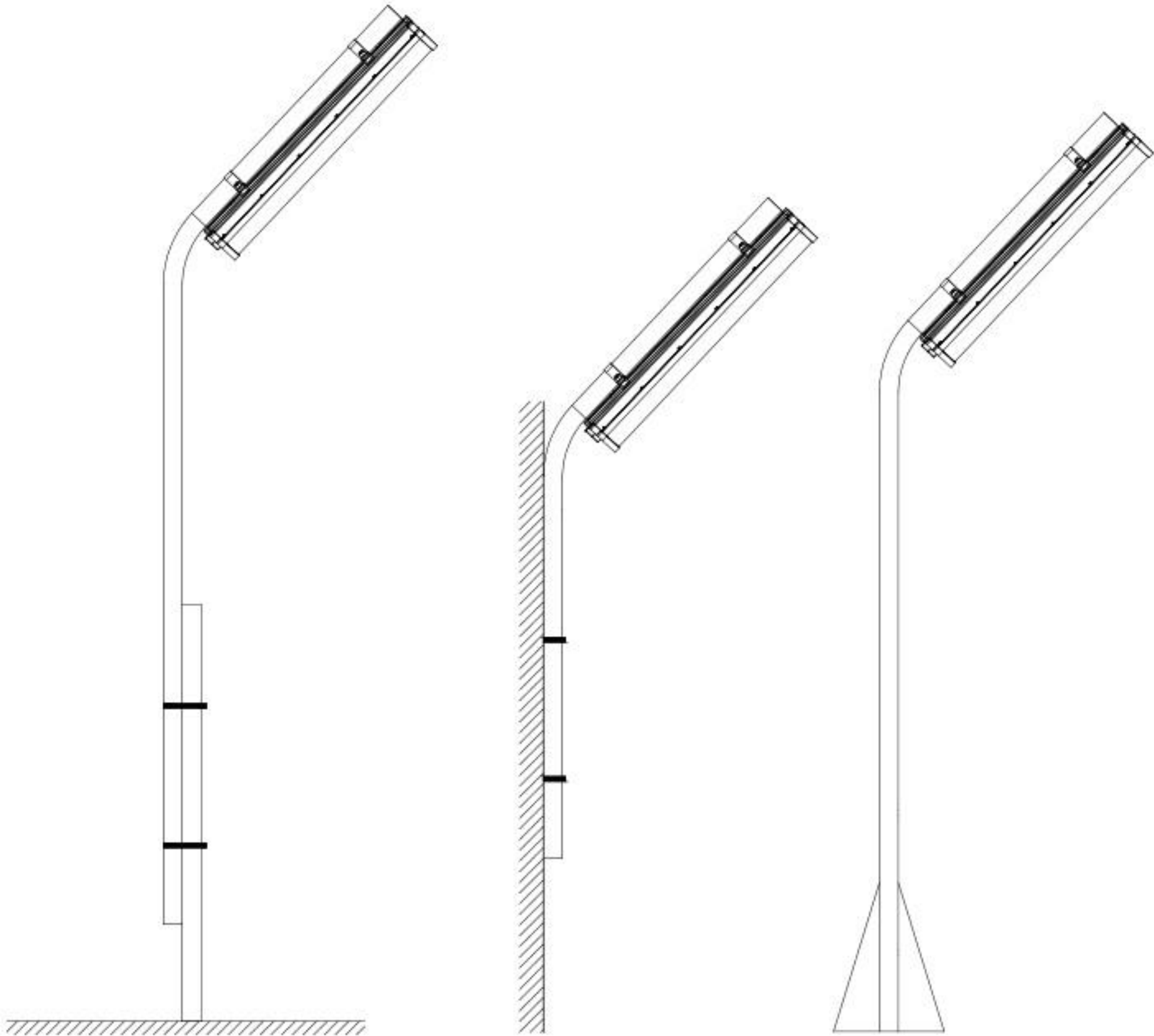
E.Pole Mounting
