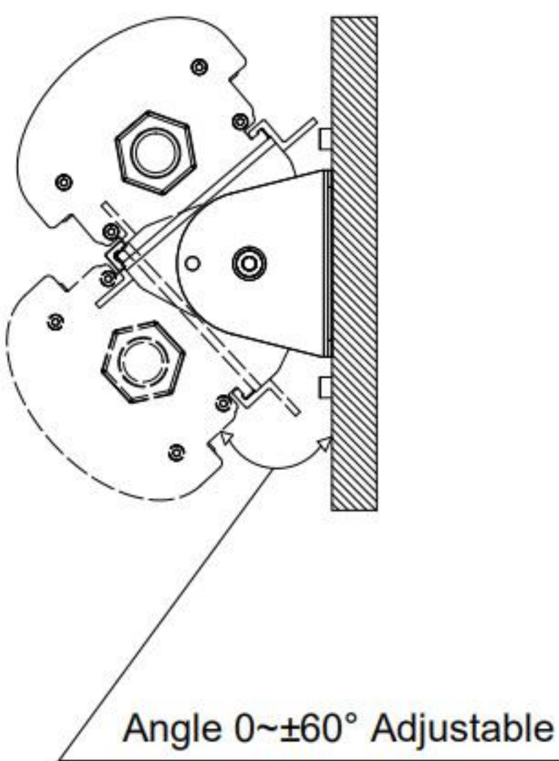
D.Wall mounting
